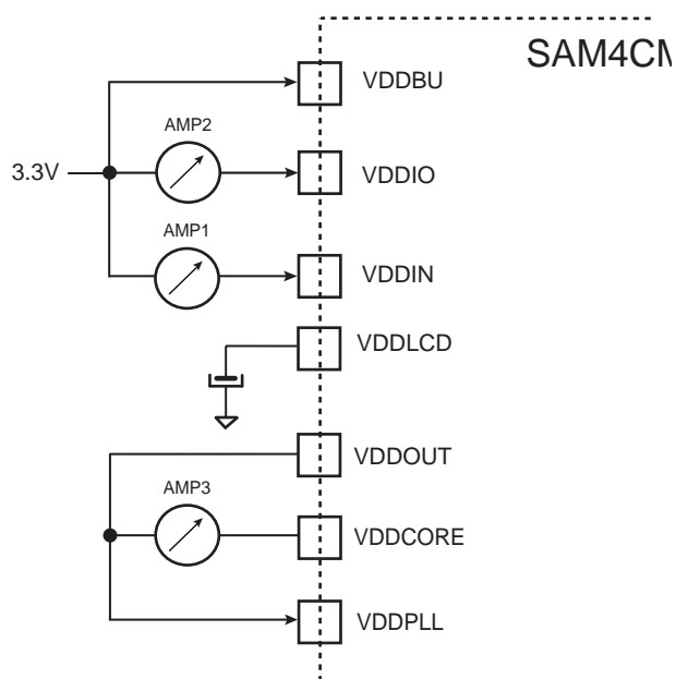
Figure 46-23. Measurement Setup for Active Mode
