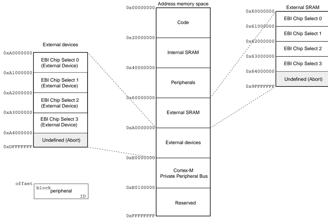
Figure 7-6. SAM4CM32/16/8 Memory Mapping of External SRAM and External Devices Area
