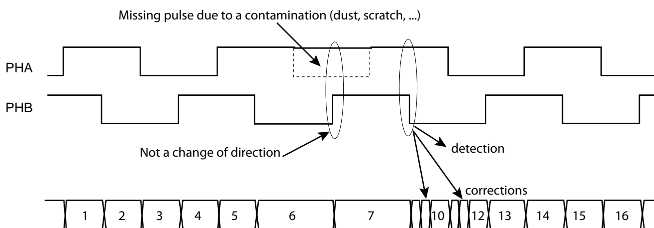
Figure 37-20. Detection and Auto-correction of Missing Pulses
