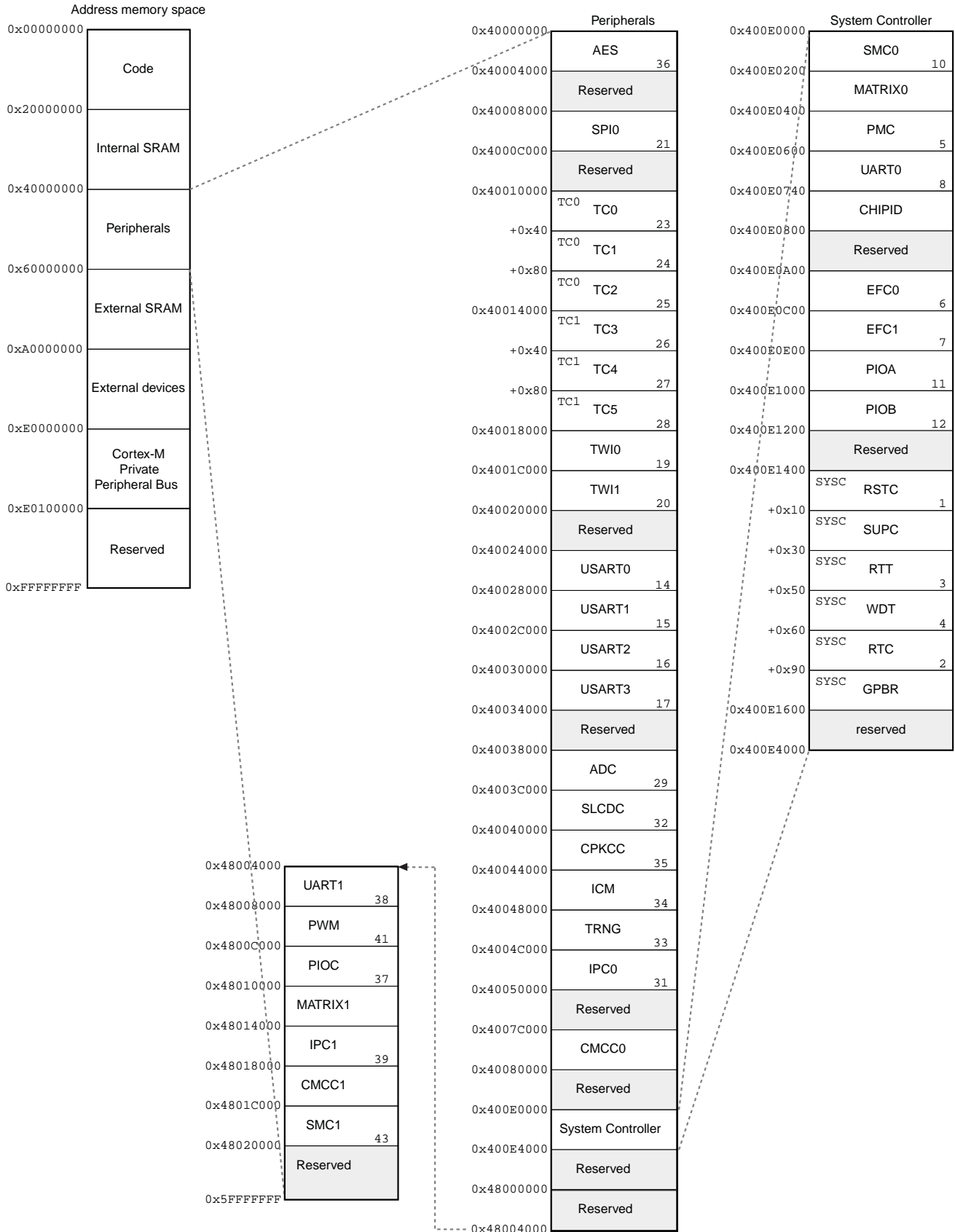
Figure 7-5. SAM4CM32 Memory Mapping of the Peripherals Area
