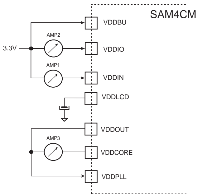
Figure 46-21. Measurement Setup for Sleep Mode
