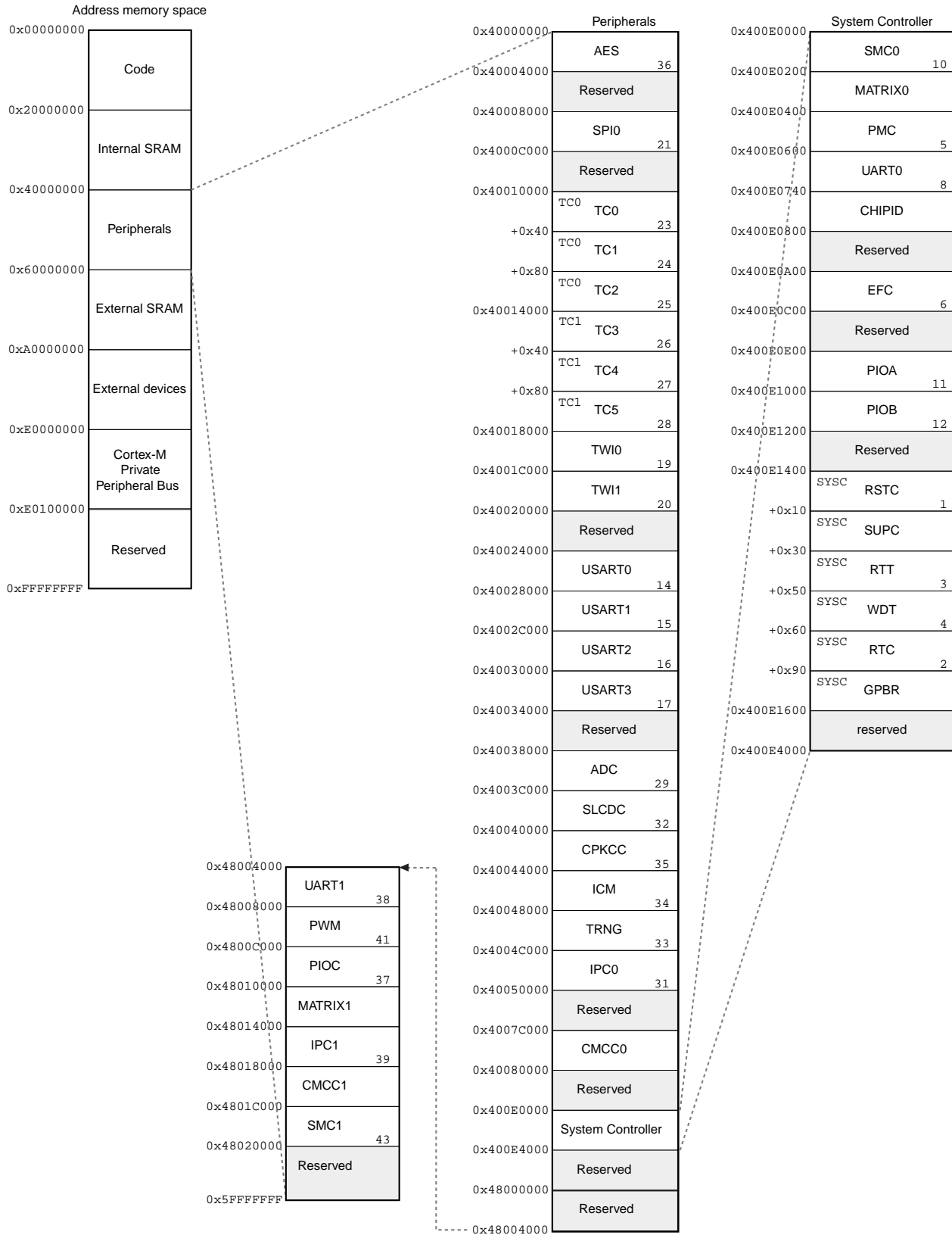
Figure 7-4. SAM4CM16/8 Memory Mapping of the Peripherals Area
