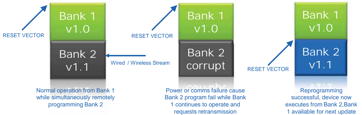
Figure 8-1. Dual Bank and Dual Boot Firmware Upgrade
