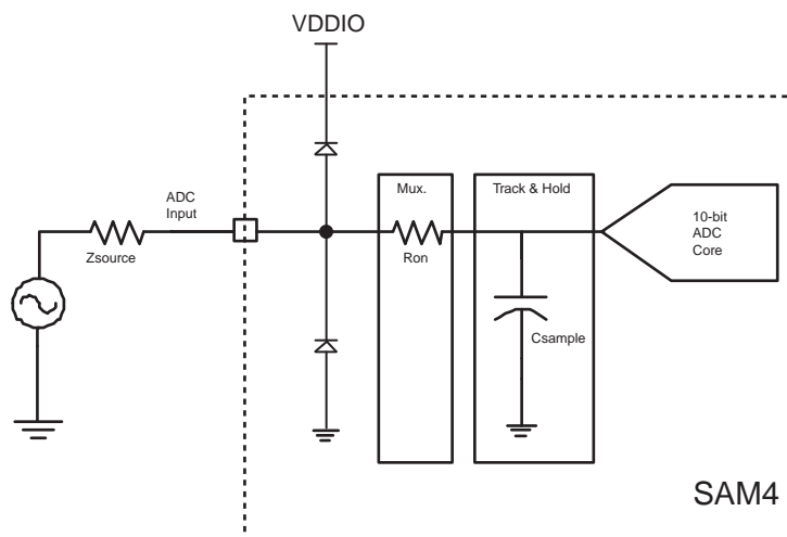
Figure 46-15. Simplified Acquisition Path
