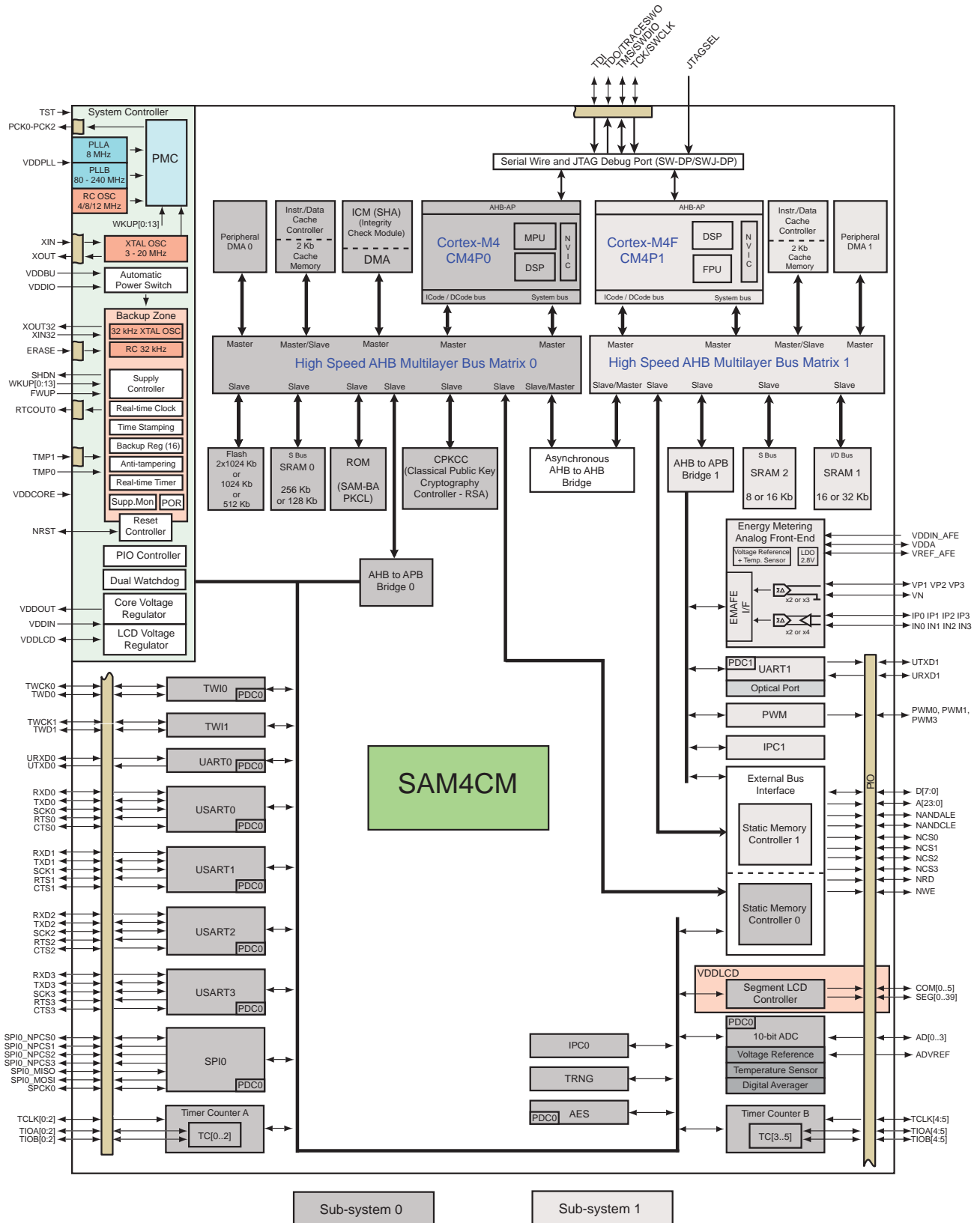
Figure 2-1. SAM4CM Series 100-pin Block Diagram
