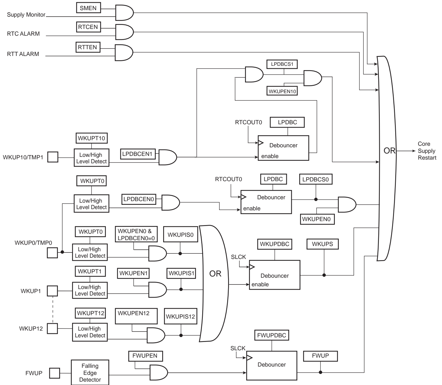
Figure 20-4. SAM4CM16/8 Wake-up Sources
