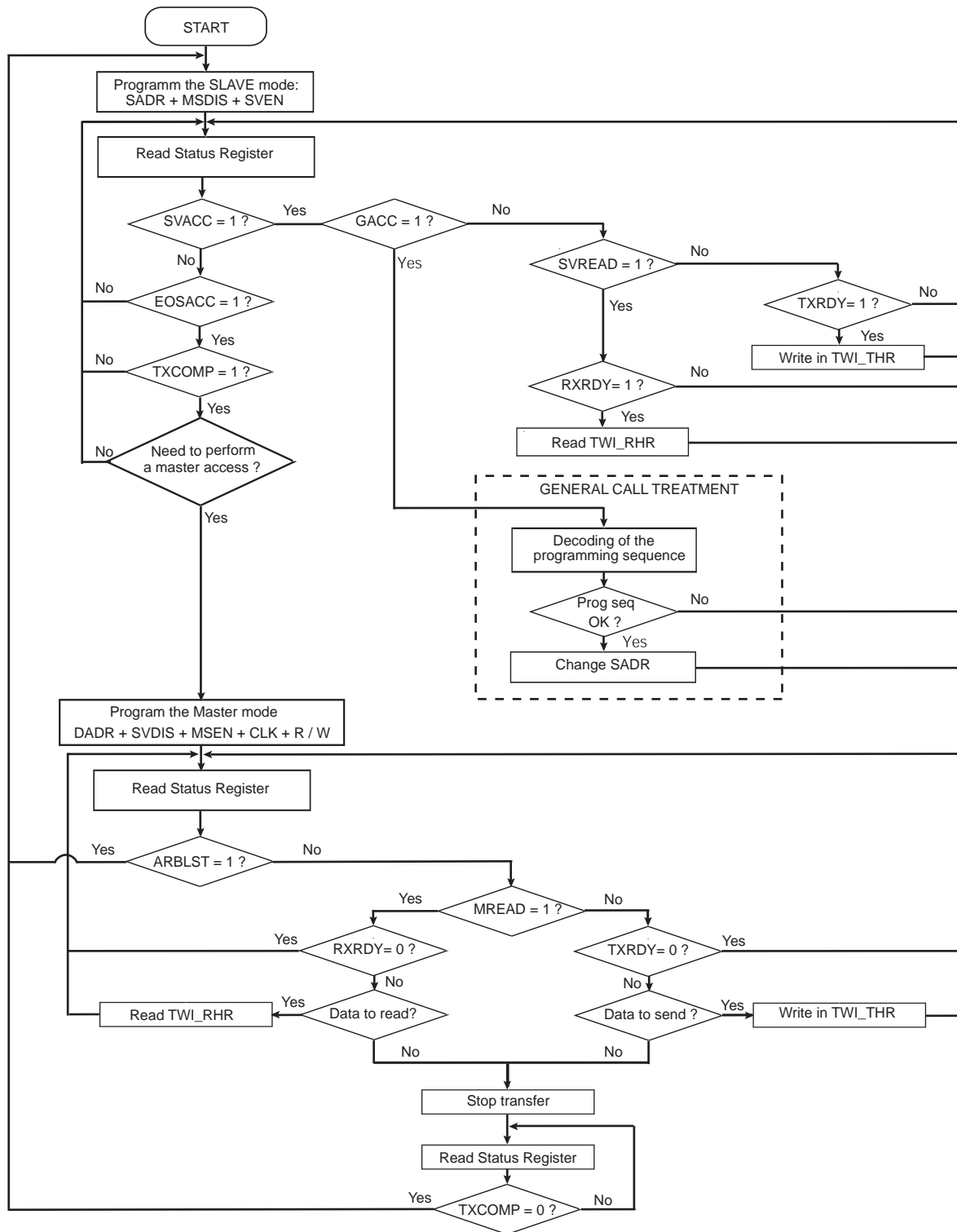
Figure 34-24. Multi-master Flowchart
