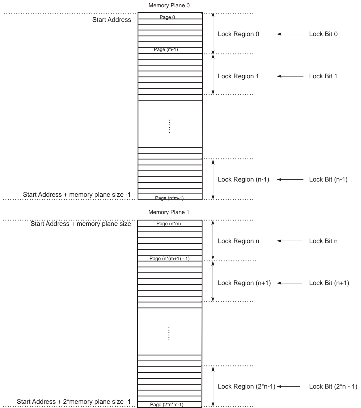
Figure 22-1. Embedded Flash Organization for Dual-plane Devices
