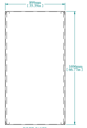
INNER PANEL
