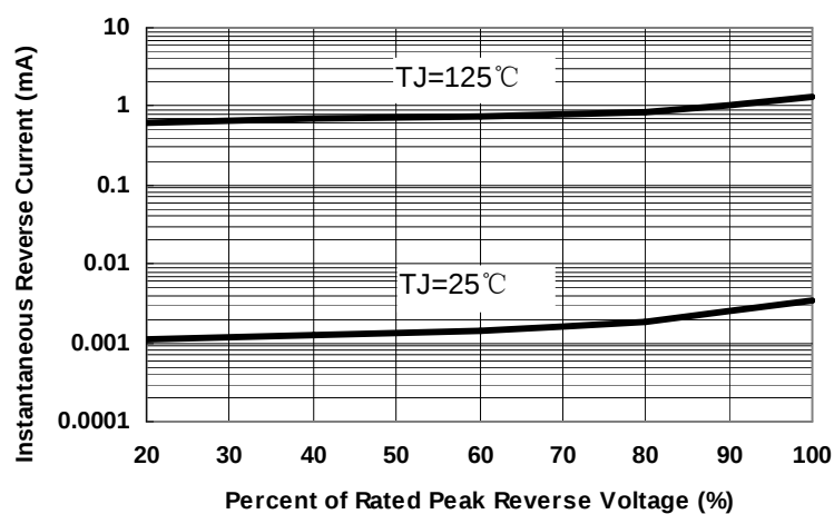
Fig.2-Typical Reverse Characteristics
