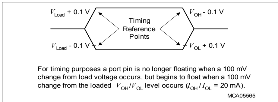
Figure 14 Floating Waveforms
