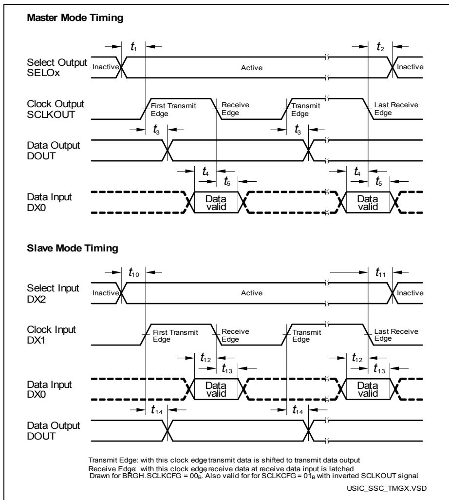
Figure 18 USIC - SSC Master/Slave Mode Timing
