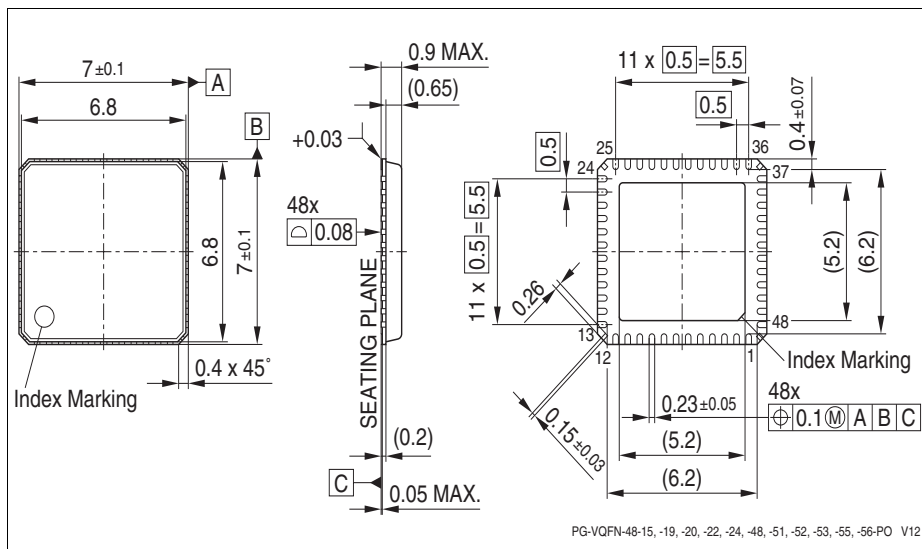
Figure 24 PG-VQFN-48-54 (Plastic Green Thin Quad Flat Package)
