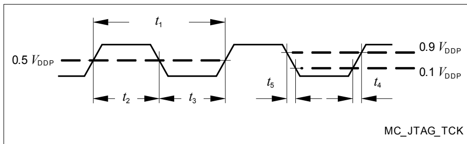
Figure 22 Test Clock Timing (TCK)
