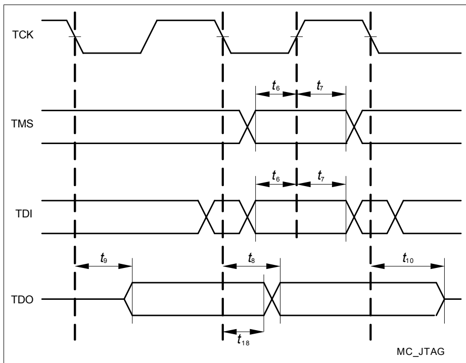
Figure 23 JTAG Timing
