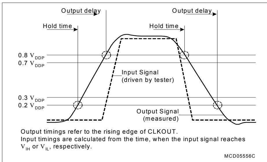
Figure 13 Input Output Waveforms
