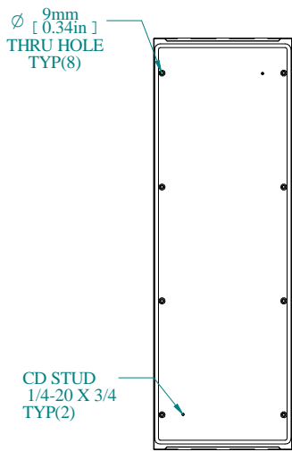
REAR VIEW
