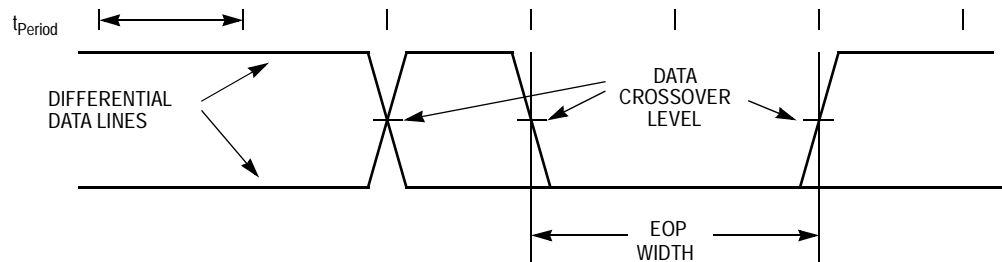
Figure 9-8. EOP Width Timing
