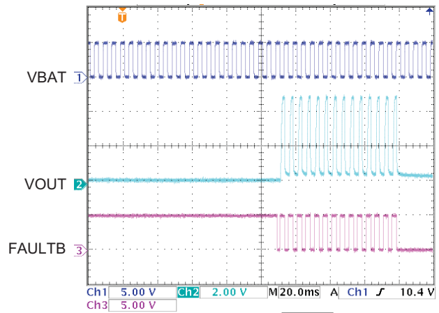
Figure 9. Battery OVP and Counter
