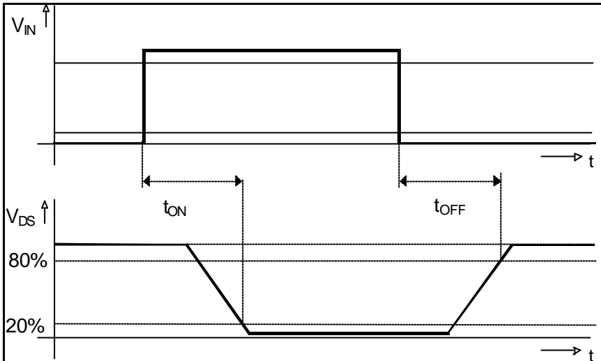
Figure 5: Power Outputs Timing is valid for resistive load with parallel and serial control. Rising edge of chip select initiates the switching
