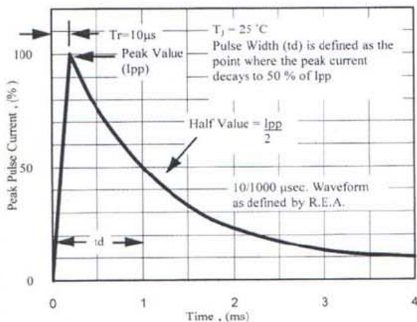
Fig. 5 - Pulse Waveform
