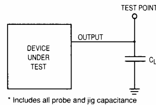
Figure 4. Test Circuit
