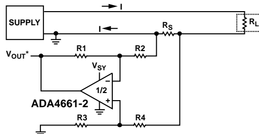
Figure 79. Low-Side Current Sensing Circuit
