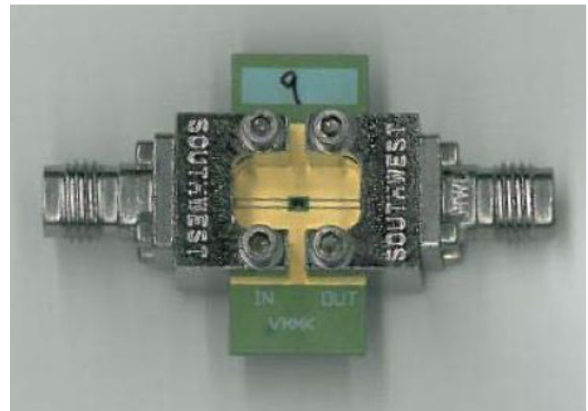
Figure 8. VMMK-3413 Characterization Board
