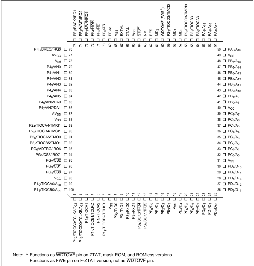
Figure 1.2 Pin Arrangement (FP-100B, TFP-100B, TFP-100G: Top View)
