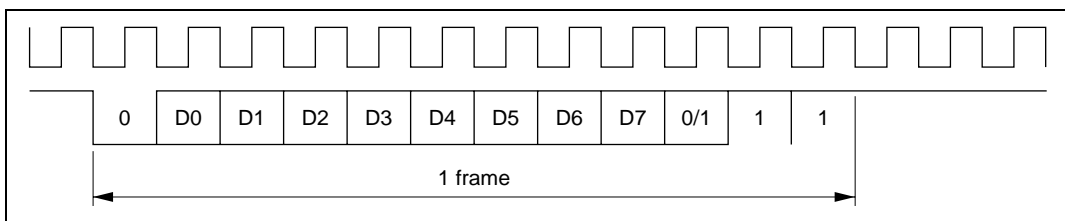
Figure 12.3 Relation between Output Clock and Transfer Data Phase (Asynchronous Mode)
