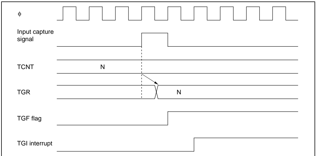
Figure 9.43 TGI Interrupt Timing (Input Capture)
