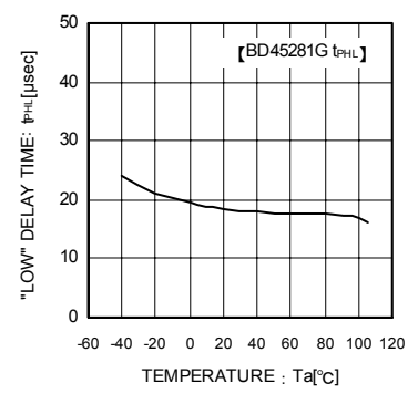
Fig.14 Output Delay Time "High" → "Low"
