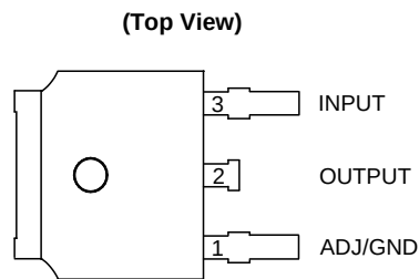
TO252-2 (3) Option 1
