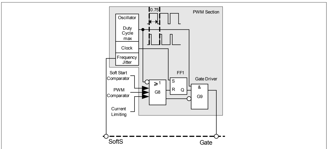
Figure 8 PWM section
