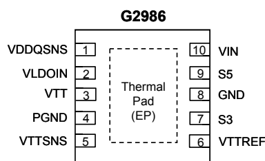
TDFN2X2-10
