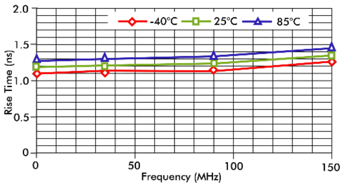
Rise Time
