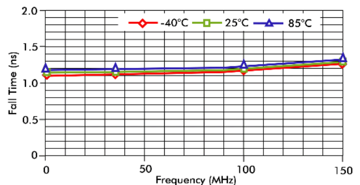
Fall Time
