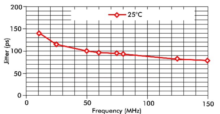
Cycle to Cycle Jitter
