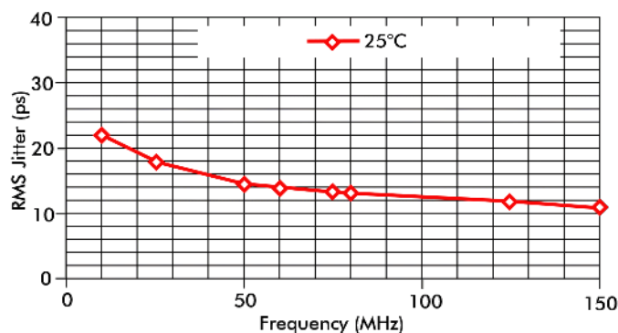
Period Jitter
