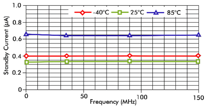
Standby Current
