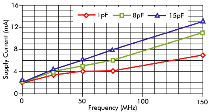
Supply Current
