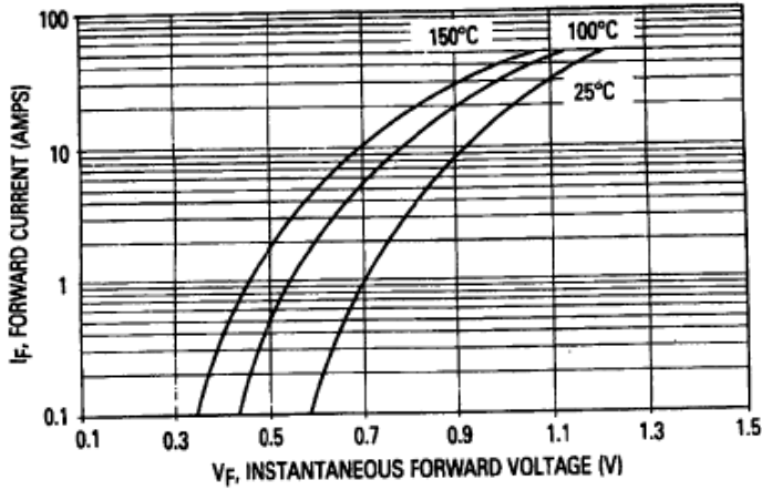
Figure 1. Typical Forward Voltage
