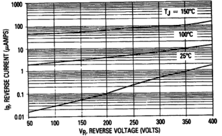
Figure 2. Typical Reverse Current
