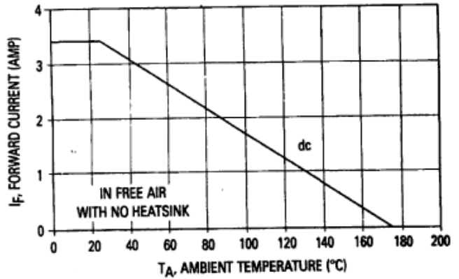
Figure 4. Current Derating, Ambient
