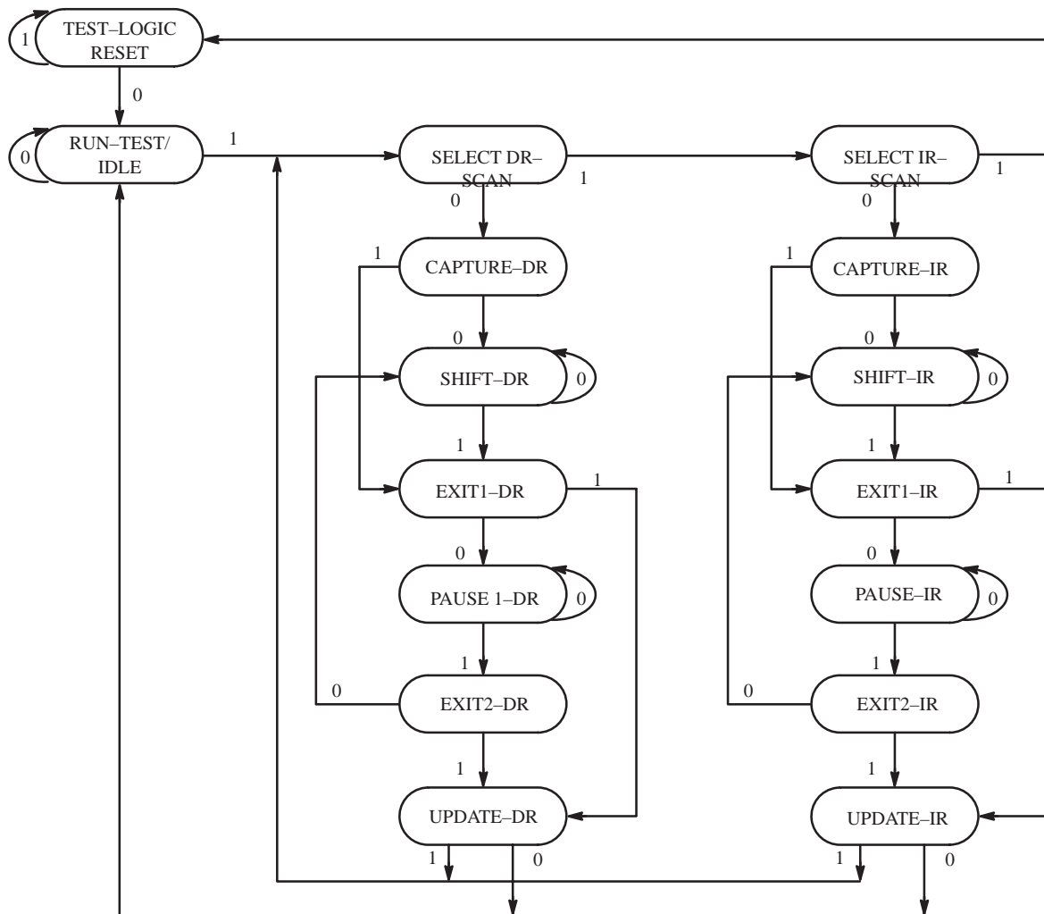
Figure 10. TAP Controller State Diagram
