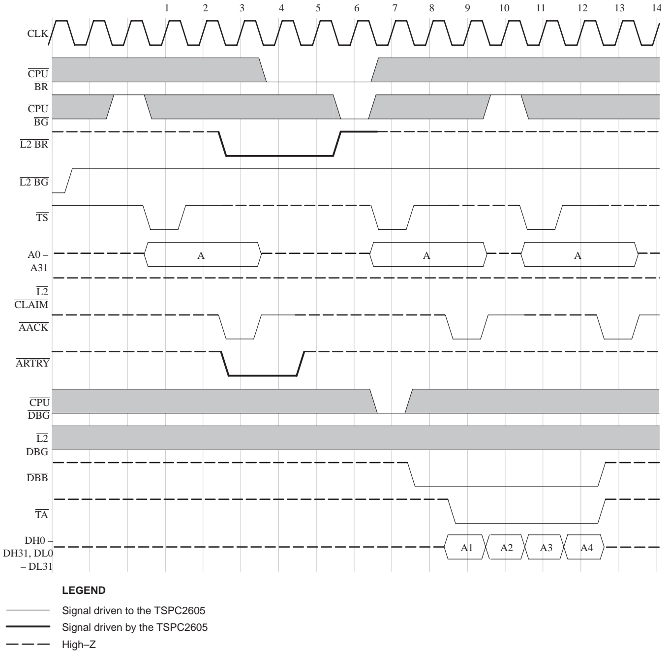
Figure 8. Read or Write Snoop Hit to Dirty L2 Cache Line and Dirty Processor Cache Line
