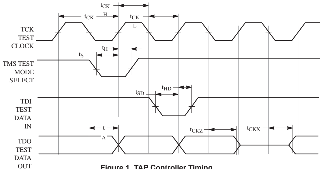
Figure 1. TAP Controller Timing
