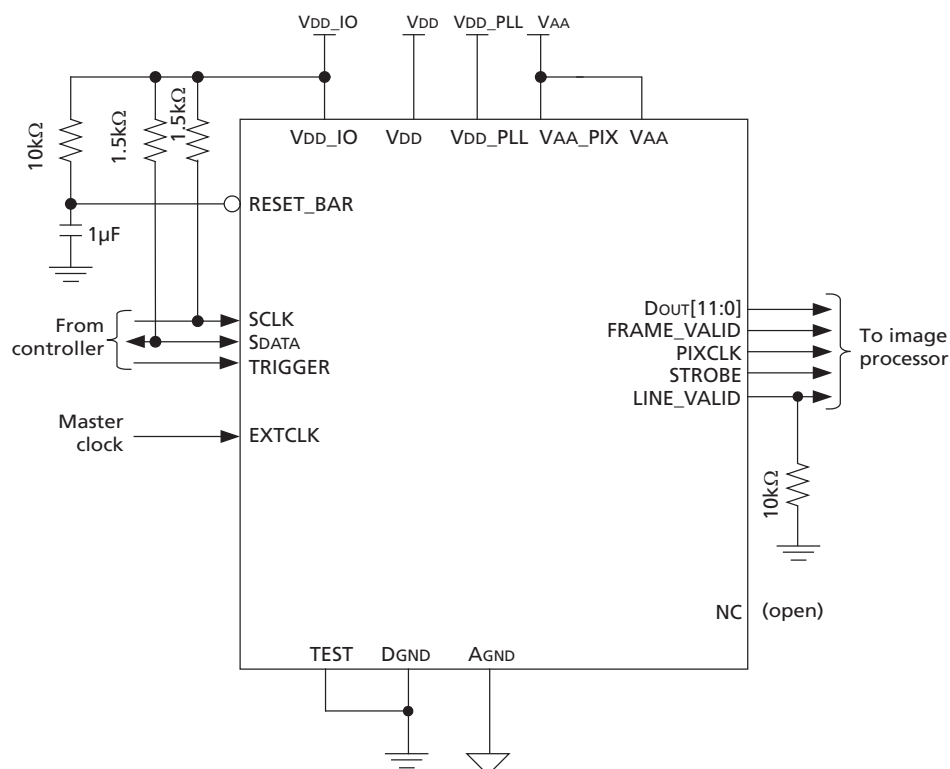
Figure 3: Typical Configuration
