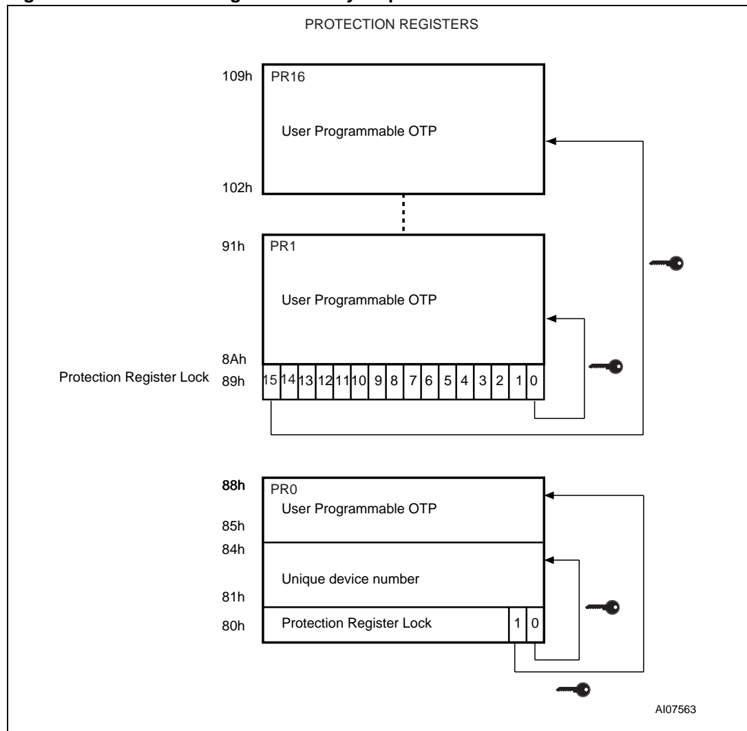
Figure 5. Protection Register memory map
