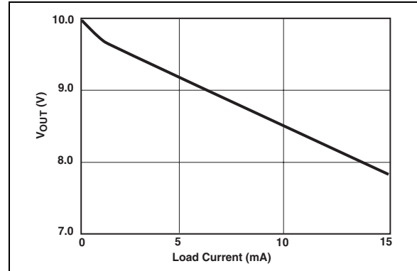
FIGURE 2-4: V_{OUT}^+ or V_{OUT}^- vs. Load Current.
