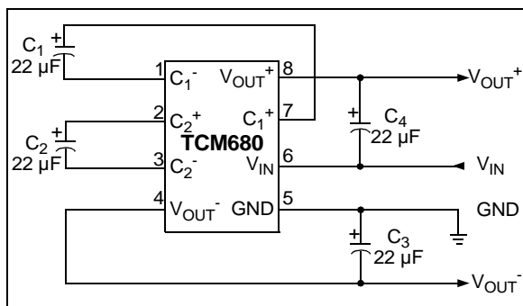
FIGURE 5-1: Positive and Negative Converter.
