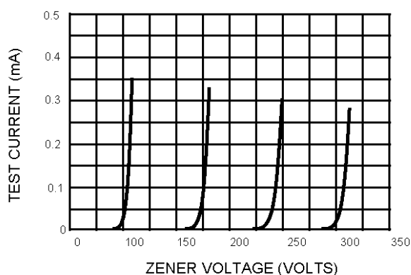
FIG. 2 - TYPICAL ZENER VOLTAGE CHARACTERISTIC
