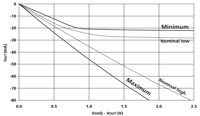
Figure 11: Reduced-Drive Pull-Up Characteristics
