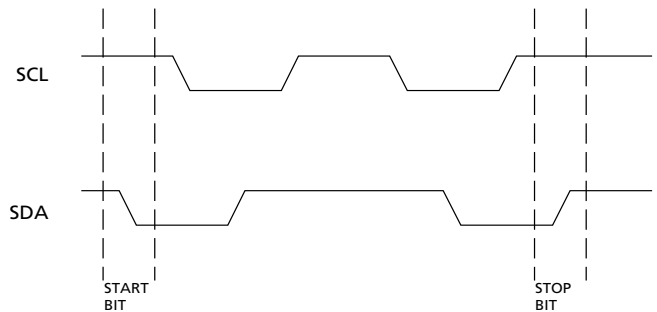
Figure 14: Definition of Start and Stop
