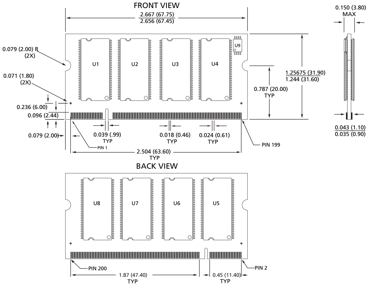
Figure 17: 200-Pin DDR SODIMM Dimensions
