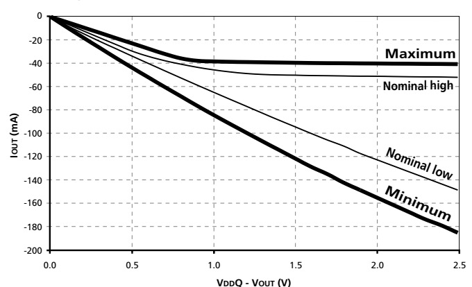
Figure 9: Pull-Up Characteristics
