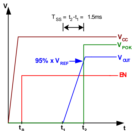
Figure 1. Soft-Start Sequence
