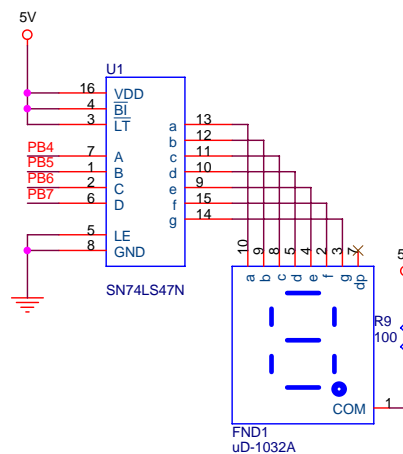
7-Segment part #1
