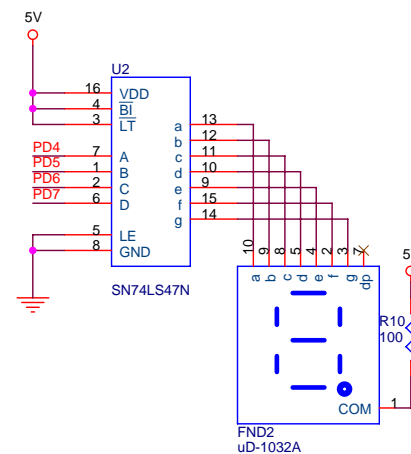
7-Segment part #2
