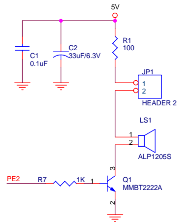
Buzzer Part
