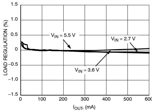
Figure 22. Load Regulation ( V_{OUT} = 1.2\text{ V} , T_A = 25^\circ\text{C} )
