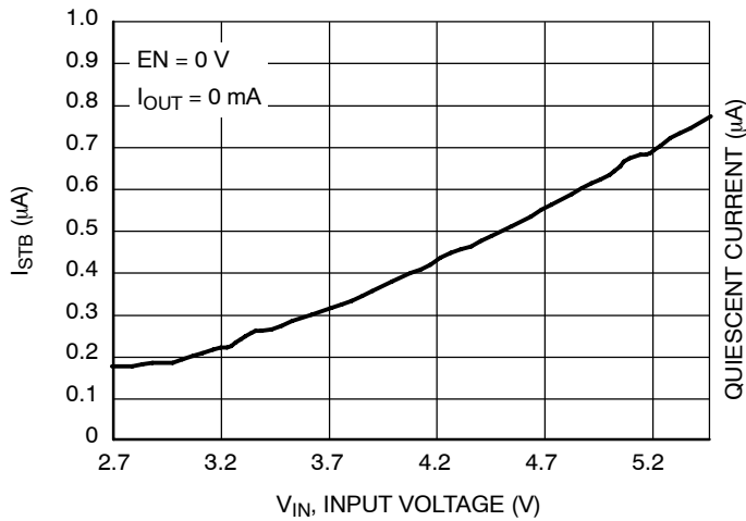
Figure 7. Shutdown Current vs. Supply Voltage
