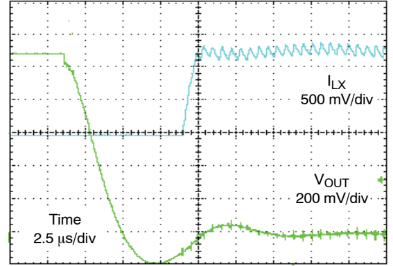
Figure 16. Short-Circuit Protection (V_{IN} = 3.6 \text{ V}, V_{OUT} = 1.2 \text{ V})
