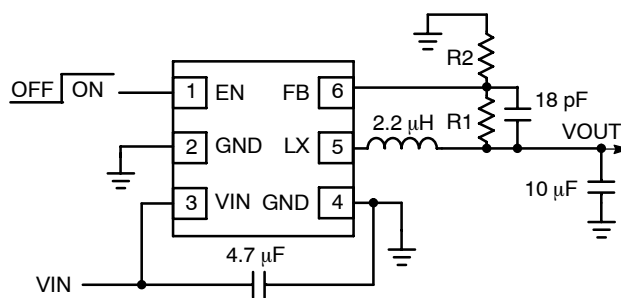
Figure 2. Typical Application - UDFN6
