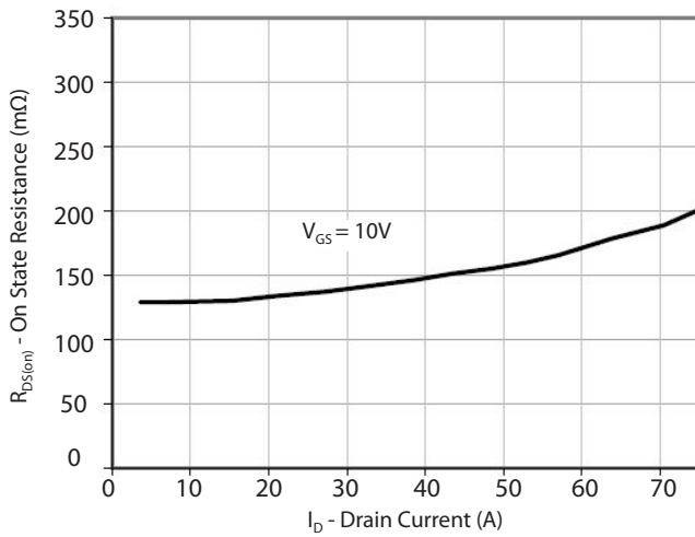
On State Resistance vs Drain Current
