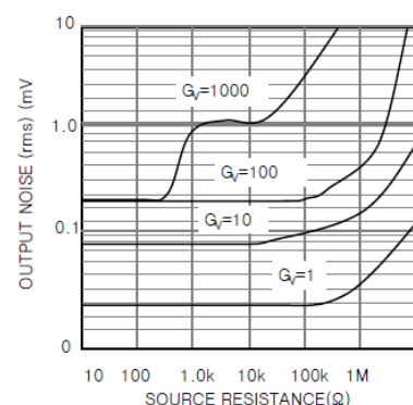
Figure 3. Output Noise vs Source Resistance
