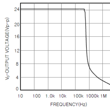
Figure 9. Power Bandwidth
