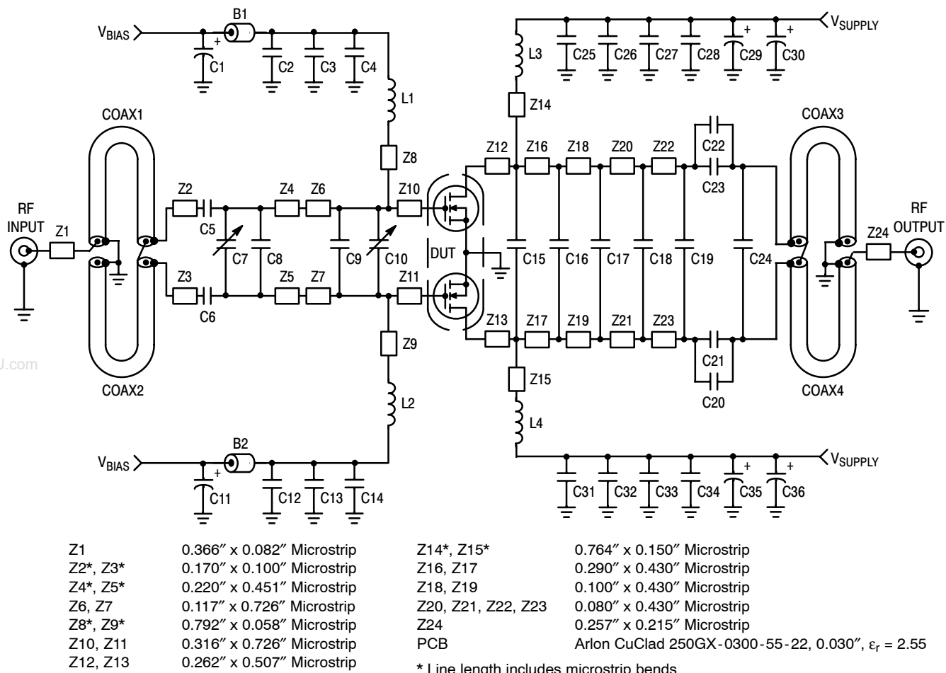
Figure 2. MRF6VP41KHR6 Test Circuit Schematic
