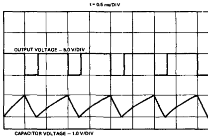
R_1 = R_2 = 4.8 \text{ k}\Omega , C_1 = 0.1 \text{ }\mu\text{F} , R_L = 1 \text{ k}\Omega
