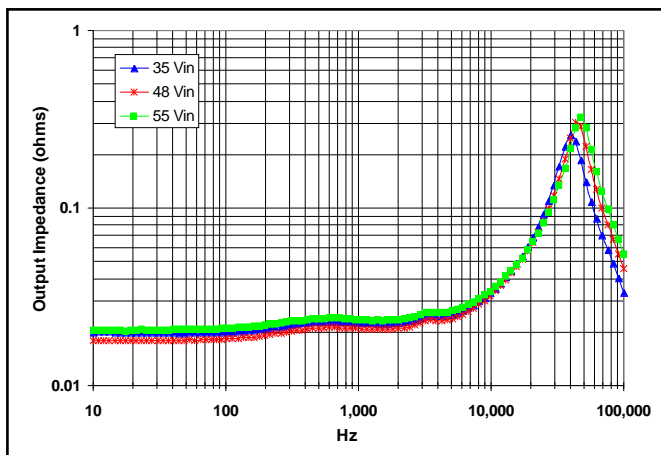
Figure 18: Magnitude of incremental output impedance ( Z_{out} = v_{out}/i_{out} ) for minimum, nominal, and maximum input voltage at full rated power.
