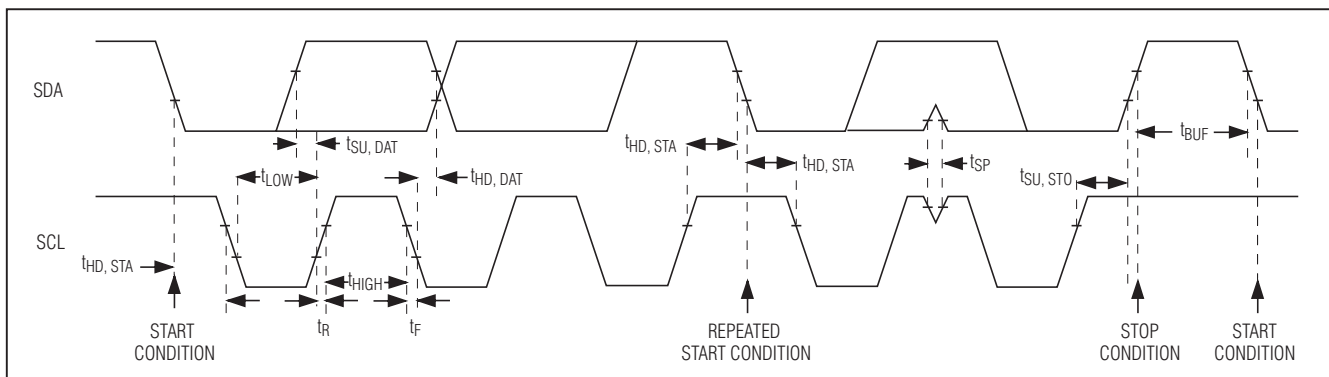
Figure 8. 2-Wire Interface Timing Diagram
