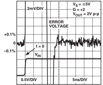
TPC 30. 0.1% Settling Time V_{OUT} = 2\text{ V p-p}
