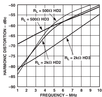
TPC 12. Harmonic Distortion vs. Frequency for Various Loads, V_S = \pm 5 V , V_{OUT} = 2 V p-p , G = +2
