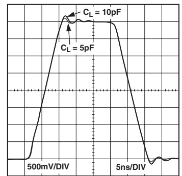
TPC 27. Large Signal Transient Response for Various Capacitive Loads, V_S = \pm 5 V
