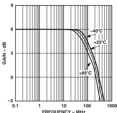
TPC 11. Frequency Response vs. Temperature, Gain = +2, V_S = \pm 5 V , V_{OUT} = 2 V p-p
