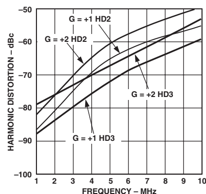
TPC 15. Harmonic Distortion vs. Frequency for Various Gains, V_S = 5 V , V_{OUT} = 2 V p-p
