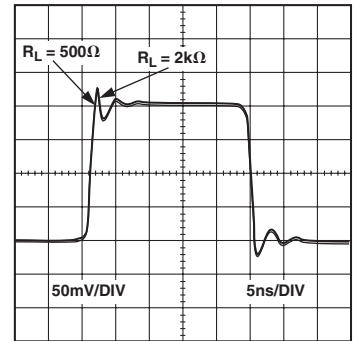
TPC 21. Small Signal Transient Response for Various R_{LOAD} , V_S = \pm 5 V
