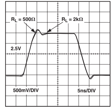
TPC 24. Large Signal Transient Response for Various R_{LOAD} , V_S = 5 V
