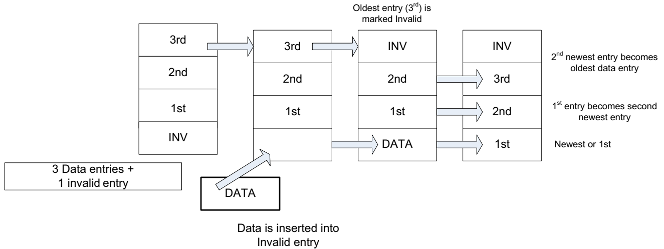
Figure 4-05. Demonstration of how entries in the received data bindings are replaced when an RF data packet is received.
