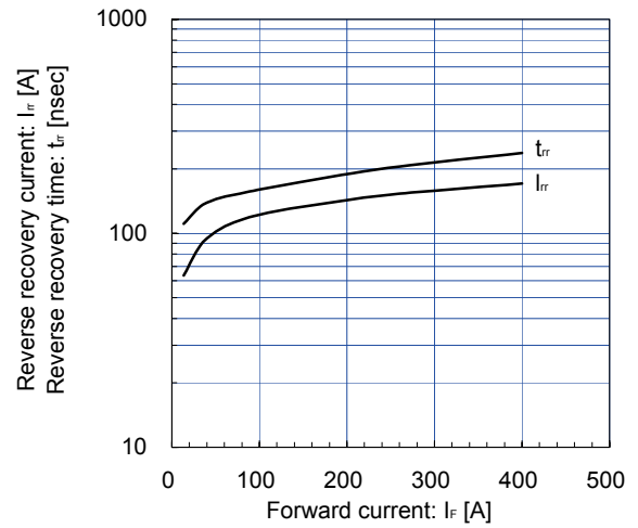
Reverse Recovery Characteristics (typ.) V_{CC}=300V, V_{GE}=\pm 15V, R_G=6.8\Omega, T_J=125^\circ C
