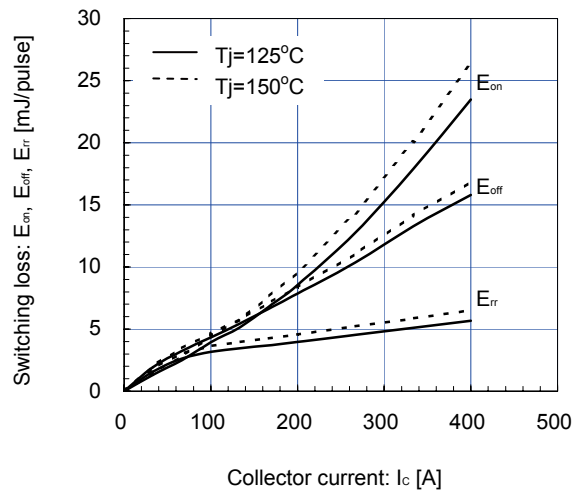
Switching loss vs. Collector current (typ.) V_{CC}=300V, V_{GE}=\pm 15V, R_G=6.8\Omega, T_J=125, 150^\circ C
