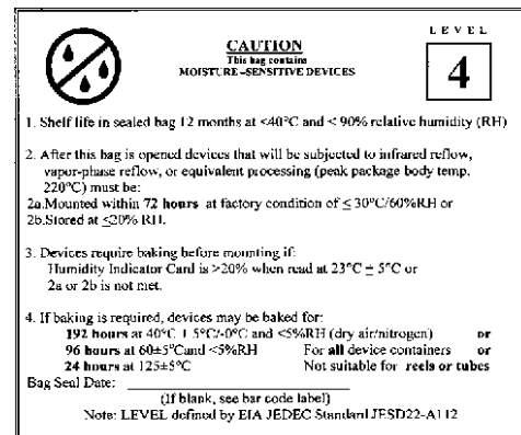
Example of JESD22-A112 level 4 label
