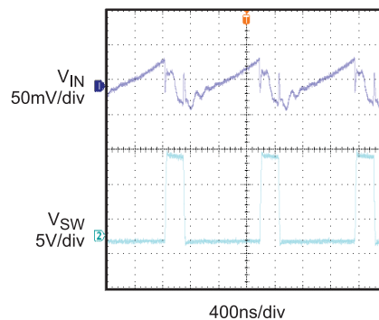
Input Ripple Voltage I_{OUT}=1.8A
