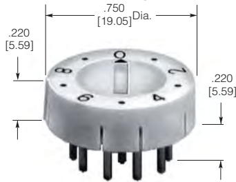
screwdriver/coin actuated Part Number 1-435097-1
