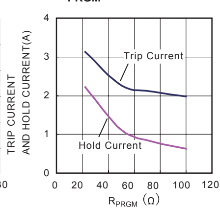
Trip Current and Hold Current vs. R_{PRGM}
