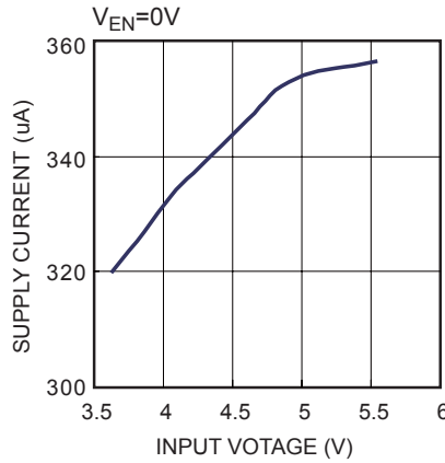
Supply Current, Output Disabled vs. Input Voltage
