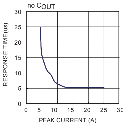
Current Limit Response Vs. Peak Current
