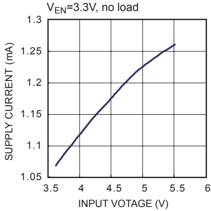
Supply Current, Output Enabled vs. Input Voltage
