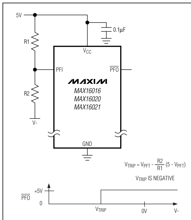
Figure 3. Monitoring a Negative Supply
