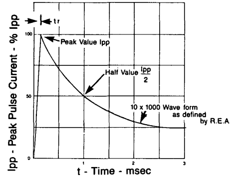
FIGURE 2 - Pulse waveform
