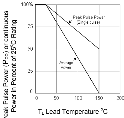
FIGURE 3 - Derating Curve
