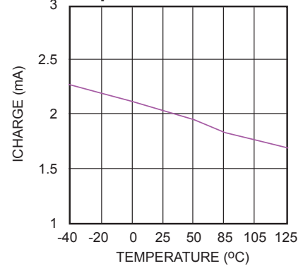
Charging Current From Pin HV (V CC =6V, V HV =400V) Vs Temperature
