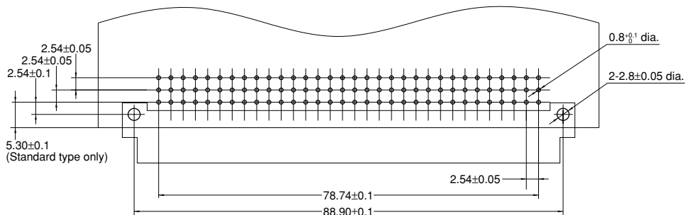
Recommended PC board pattern (Bottom view)
