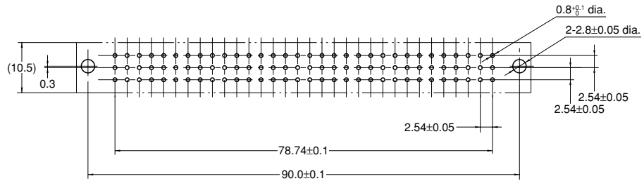
Recommended PC board pattern (Bottom view)
