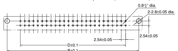
Recommended PC board pattern (Bottom view)
