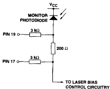
Figure 2. Back Facet Monitor Circuitry.
