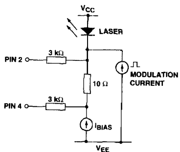
Figure 1. Laser Bias Monitor Circuitry.
