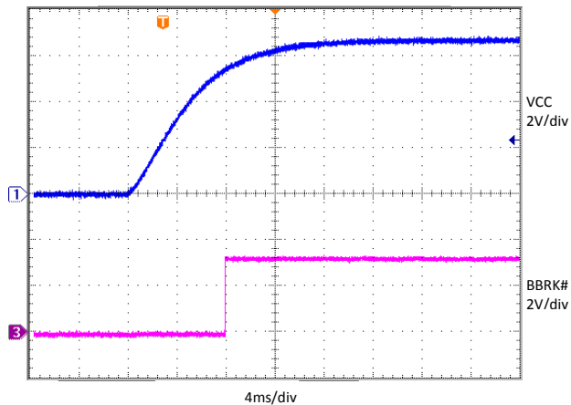
Figure 26: Diode Emulation Setup through BBRK# Input
