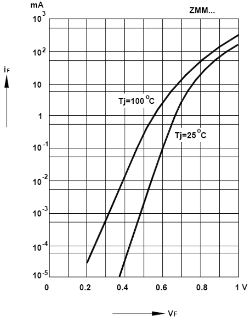
Forward characteristics
