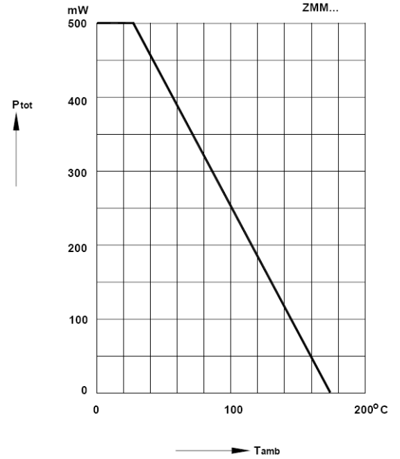
Admissible power dissipation versus ambient temperature
