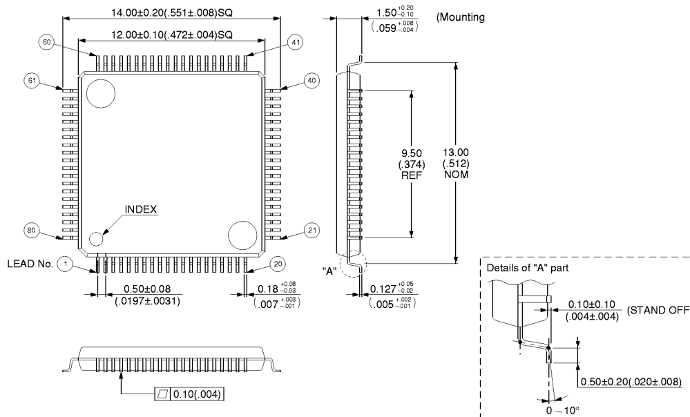
80-pin Plastic SQFP (FPT-80P-M05)
