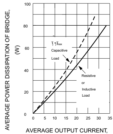
FIG.6-MAXIMUM POWER DISSIPATION
